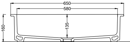
SECTION
