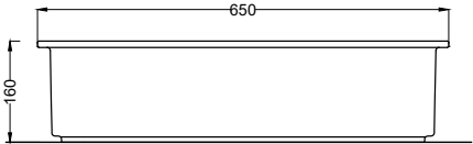
FRONT
