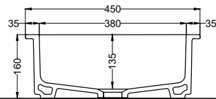
SECTION
